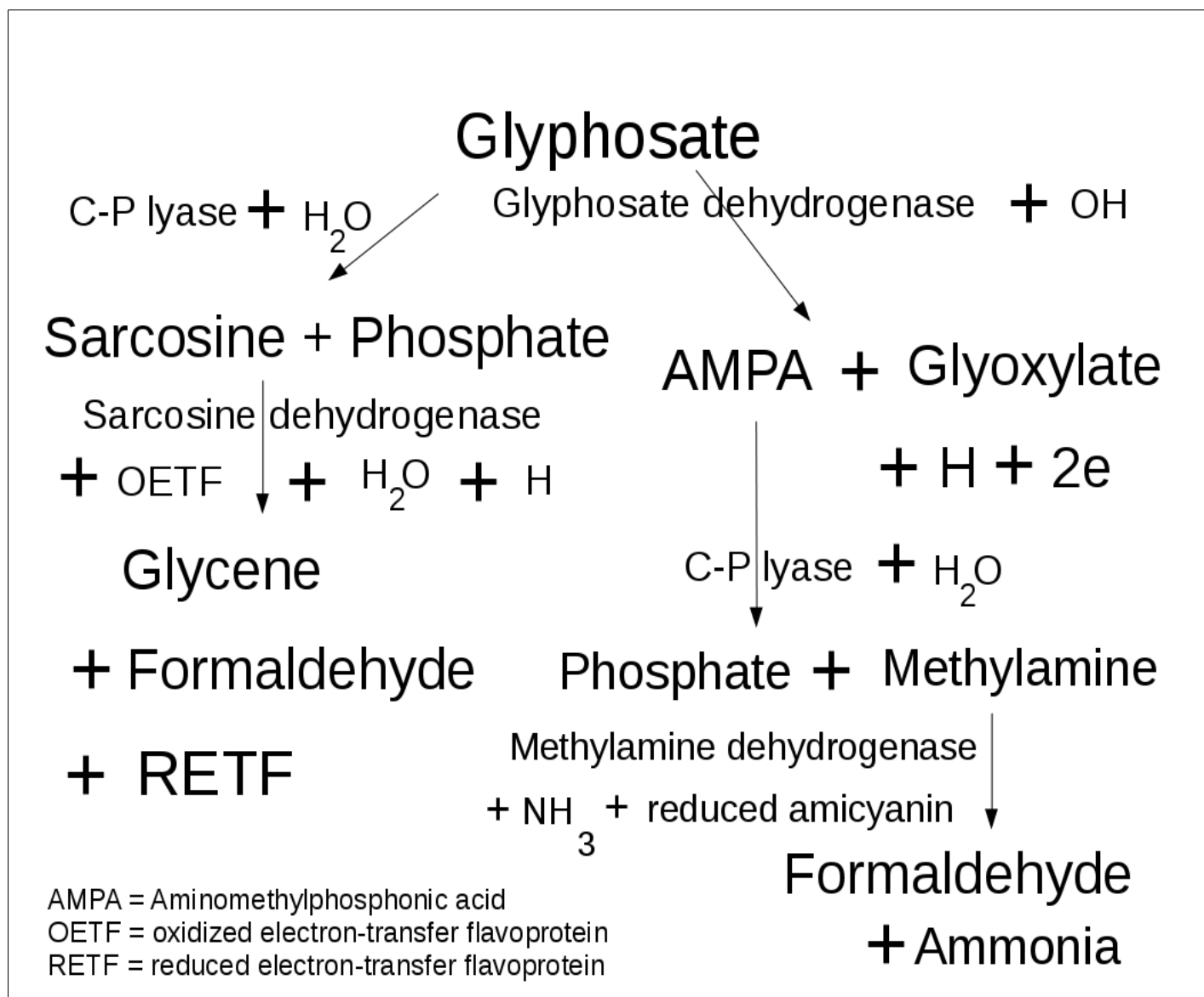
Figure 2. Possible metabolic pathways for glyphosate.
