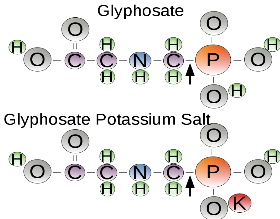
Figure 1. Glyphosate and glyphosate potassium salt molecules.
